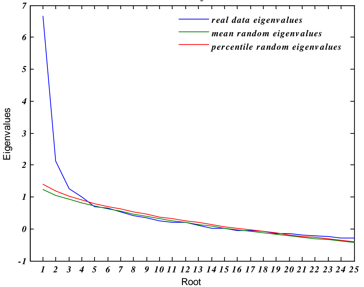
Figure S2. Real and Random-Data Eigenvalues for N-Roots based on Parallel Analysis
