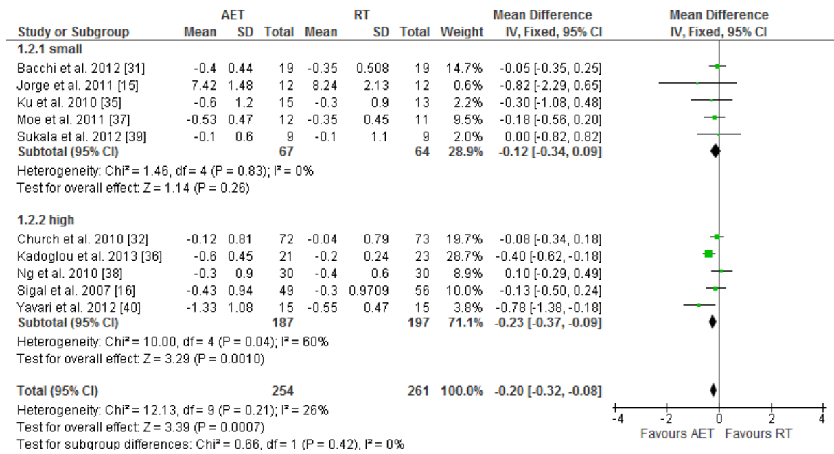
ESM Figure 17. Forest plot (small vs. high sample size) showing pooled MD with 95% CI for glycosylated haemoglobin (%) for 10 randomized aerobic training (AET) vs. resistance training (RT) groups.
